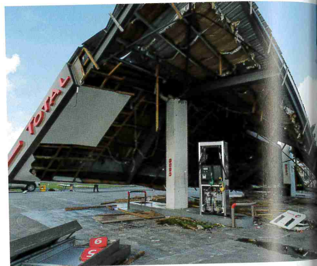
▲ Figure 5 Damaged caused by strong winds, Cyclone Winston, Fiji, 2016
