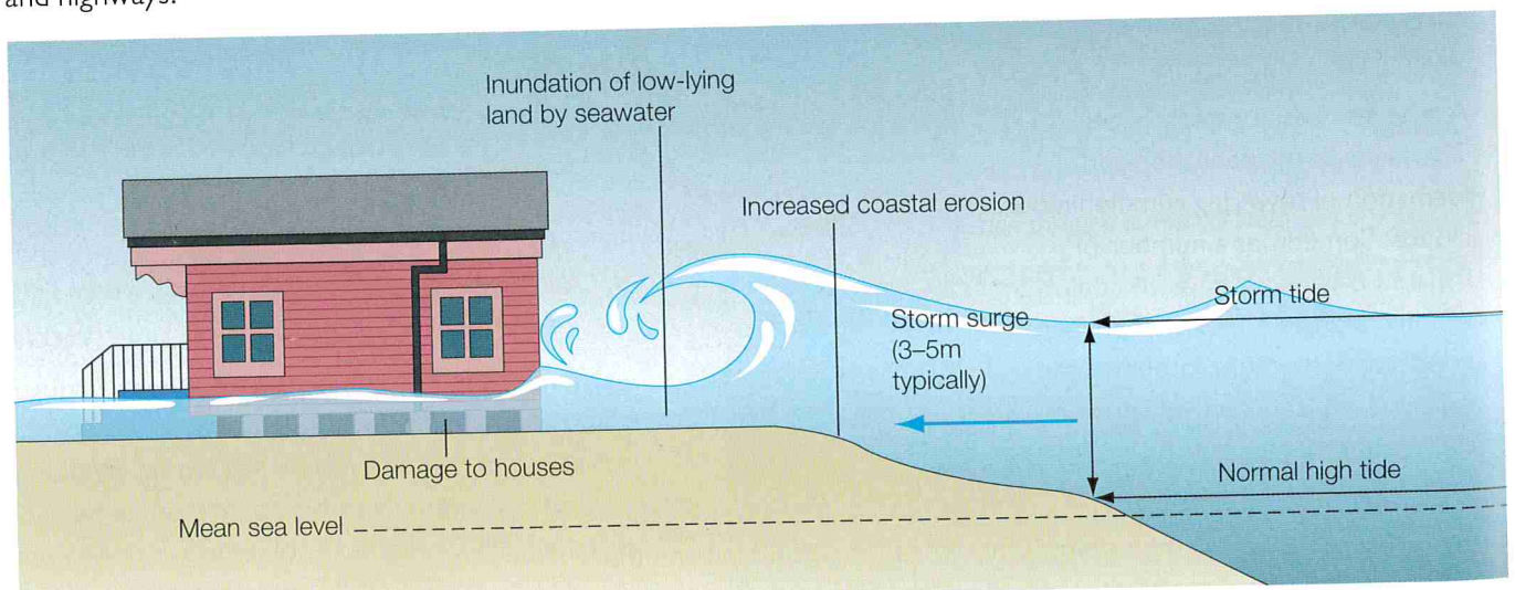
▲ Figure 6 The impact of a storm surge on a coastline
