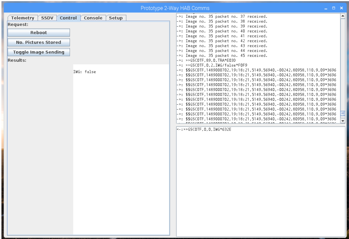
Figure 24 - Shows the transmission of the IMG packet to toggle image sending and the response 'false' shows that image transmission is now set to false.
