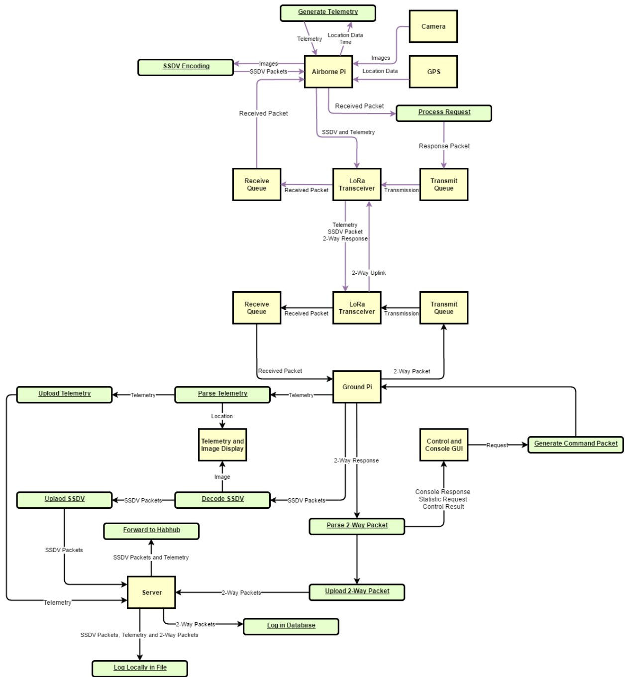
Figure 17 - Data Flow Diagram for Proposed System
