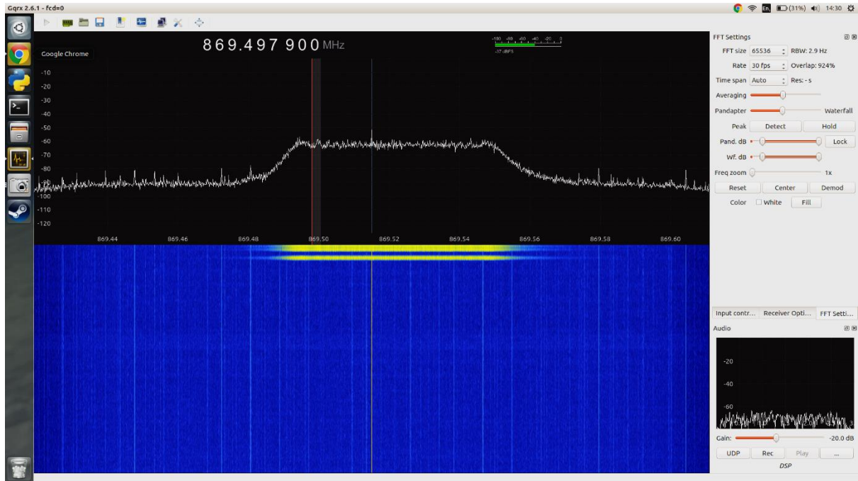
Figure 29 - Showing Gqrx, an SDR (Software Defined Radio) software, analysing what is being transmitted at 869.525MHz during testing. The difference between the frequency of the left of the peak and the frequency of the right of the peak is roughly 60-65kHz (depending on where you determine the edges to be).
