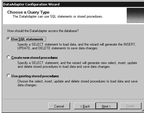
Figure 6.5 Choosing to use a SQL statement for this command.
