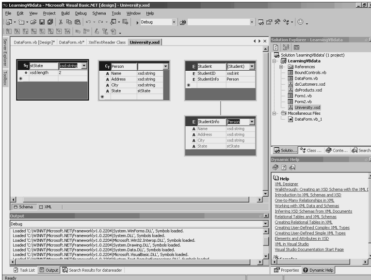
Figure 6.16 The XML Designer after you have created your schema.
